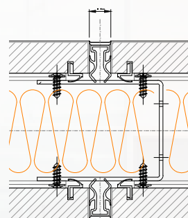
SOLID PANEL MODULE TO MODULE
