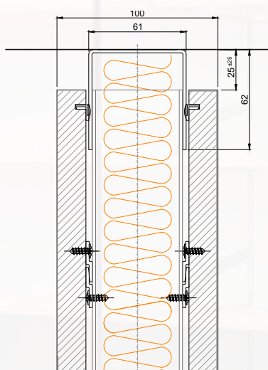
SOLID PANEL HEAD TRACK CAPABLE OF \pm 25 MM DEFLECTION
