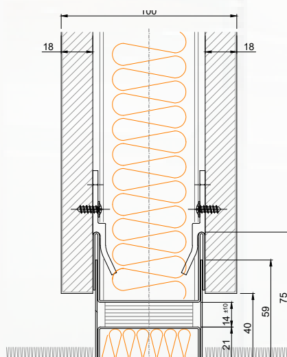
SOLID PANEL FLOOR TRACK
