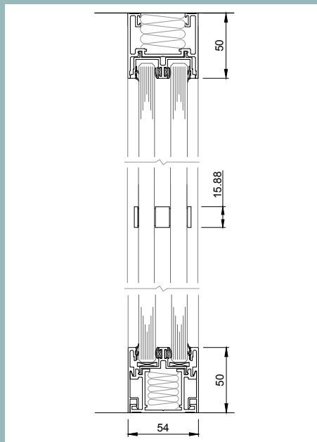
Vertical section through Revolution 54 double glazed Shoreditch screen
